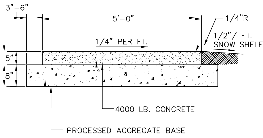
TYPICAL SECTION 5" CONCRETE SIDEWALK
