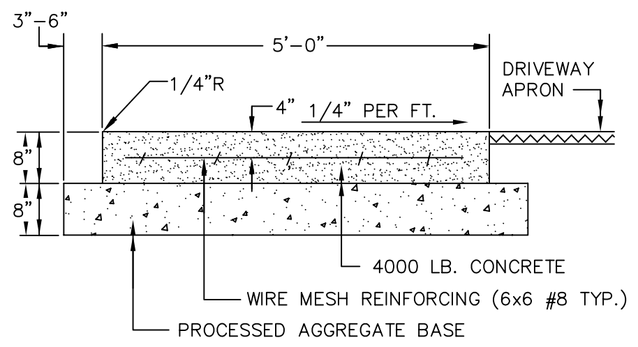
TYPICAL SECTION 8" CONCRETE SIDEWALK (DRIVEWAY)
