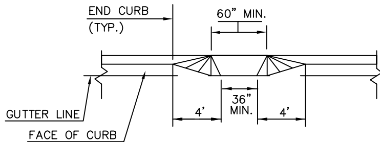
FRONT SIDEWALK RAMP
