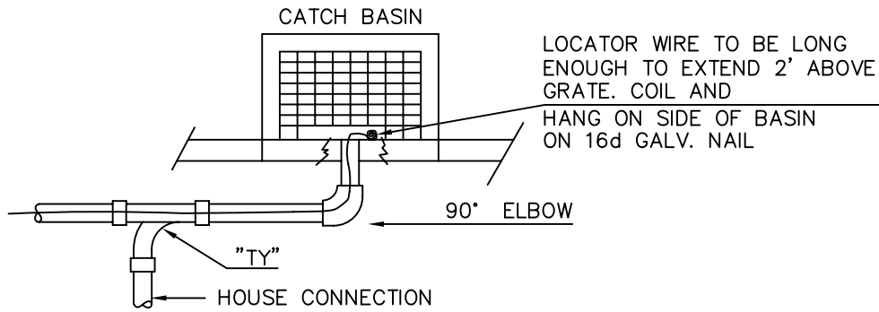
COLLECTOR / UNDERDRAIN DETAIL
