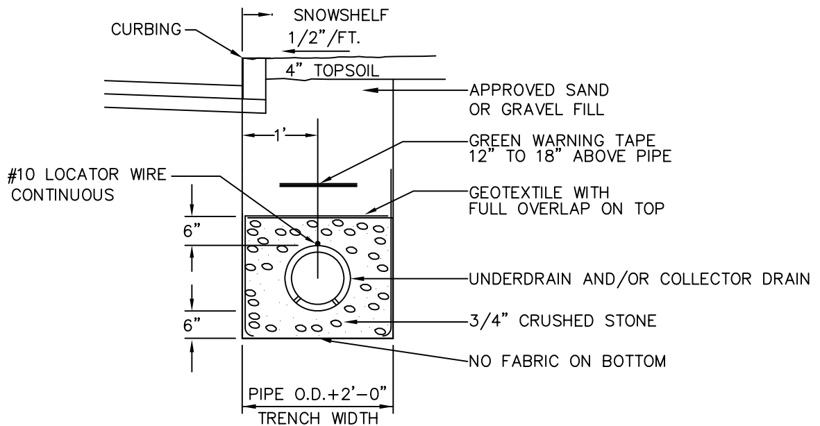
TRENCH DETAIL
