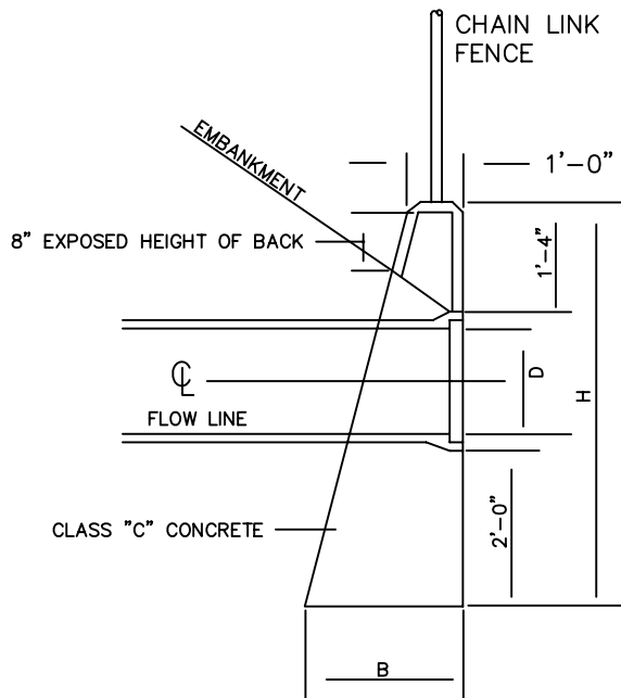
WALL AT FOOT OF SLOPE
