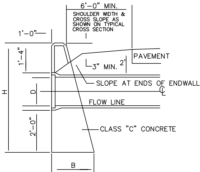
WALL AT SHOULDER
